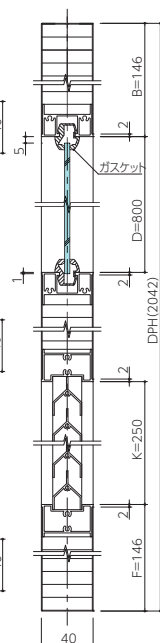
E-E'
